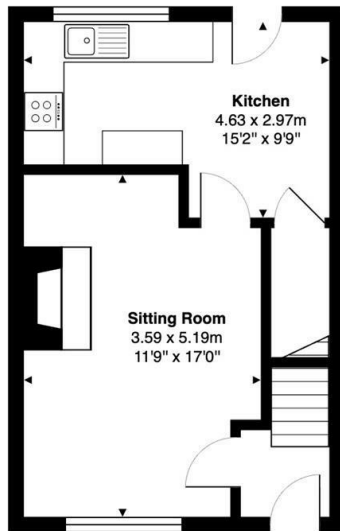
Ground Floor Gross Internal Area: 34.8 m² ... 375 ft²
